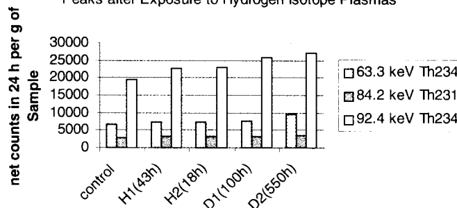
Fig. 5. Th 231 and Th 234 Characteristic Gamma Ray Peaks after Exposure to Hydrogen Isotope Plasmas
