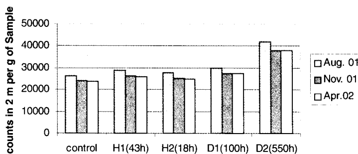
Fig. 4. Gamma Radiation from Uranium Samples after Exposure to Hydrogen Isotope Plasmas
