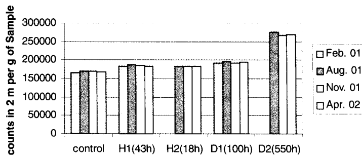
Fig. 3. Beta Radiation from Uranium Samples after Exposure to Hydrogen Isotope Plasmas
