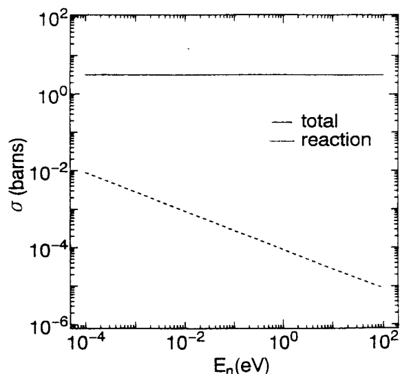
Fig. 1 Fusion and total cross section (barns) of neutron (energy E_n in eV) with a deuteron extrapolated to lower energy using the optical model.
